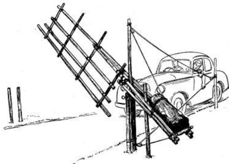
Counterpoise Gate.
