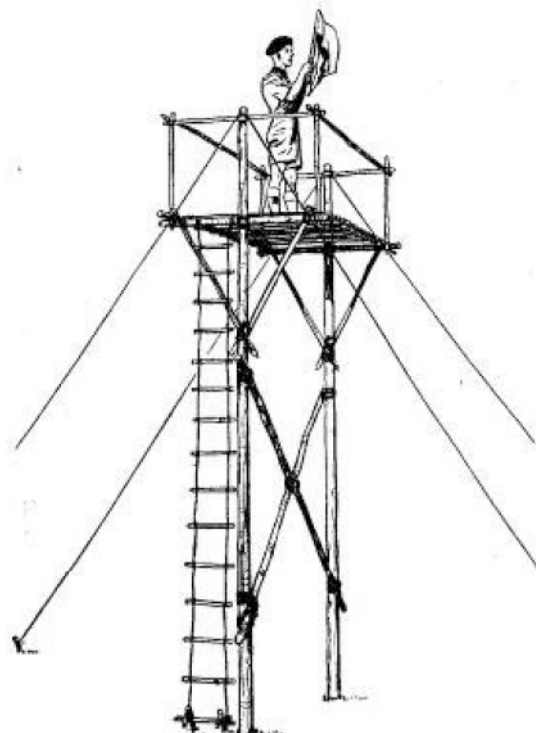
Stilt Tower.
